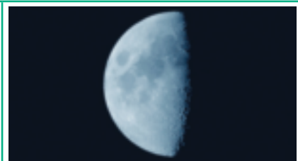
Half moon
