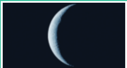
Crescent moon
